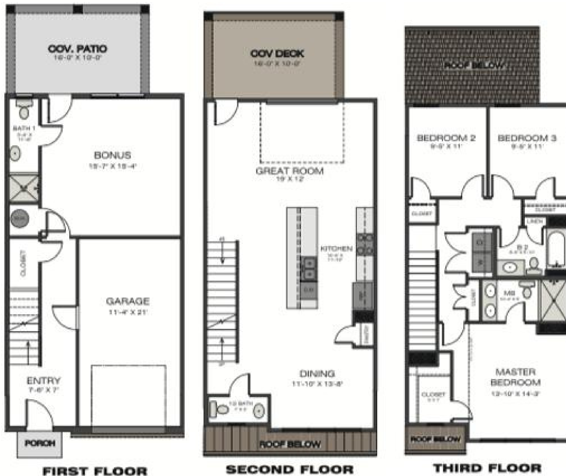
3 Bedroom Plan
