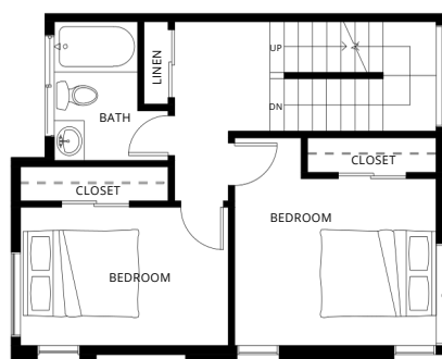
Guest Floor
